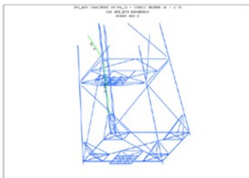
Figure 11.1-1 Member UC Plots - Jacket Bottom Section (UC-0.76)
